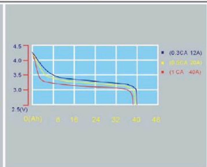
TS-LFP40AHA DISCHARGE AT TEMPERATURE OF 25°C
