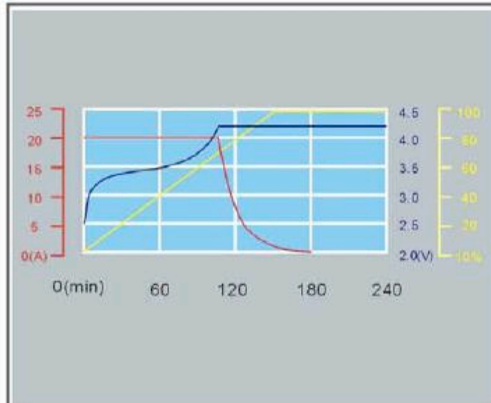
TS-LFP40AHA CHARGE AT TEMPERATURE OF 25°C
